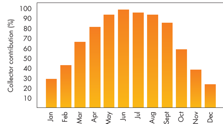
Typical solar hot water generation over a year (average of 70%)
